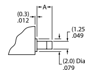
Standoff Detail
